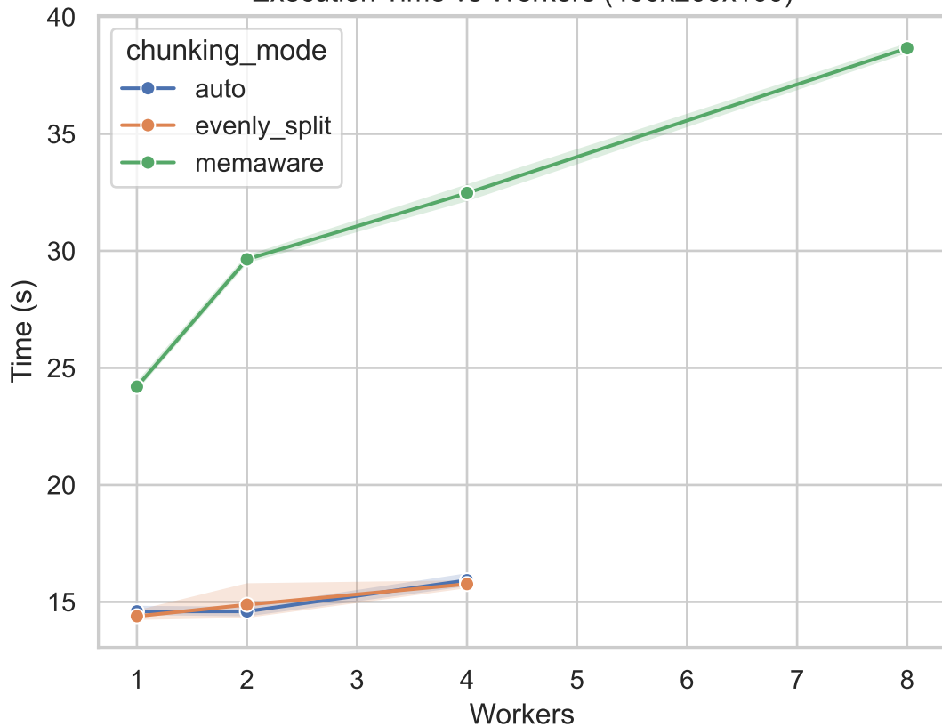
Execution Time vs Workers (400x200x100)
