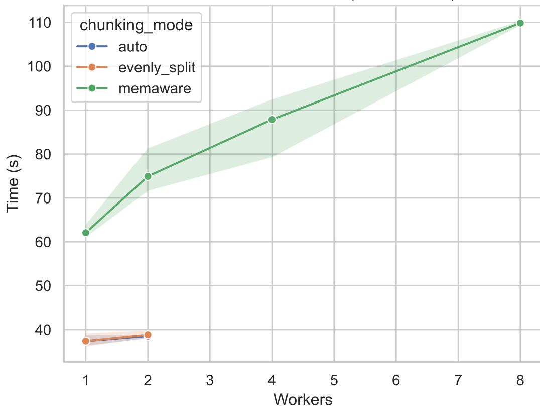
Execution Time vs Workers (400x200x300)
