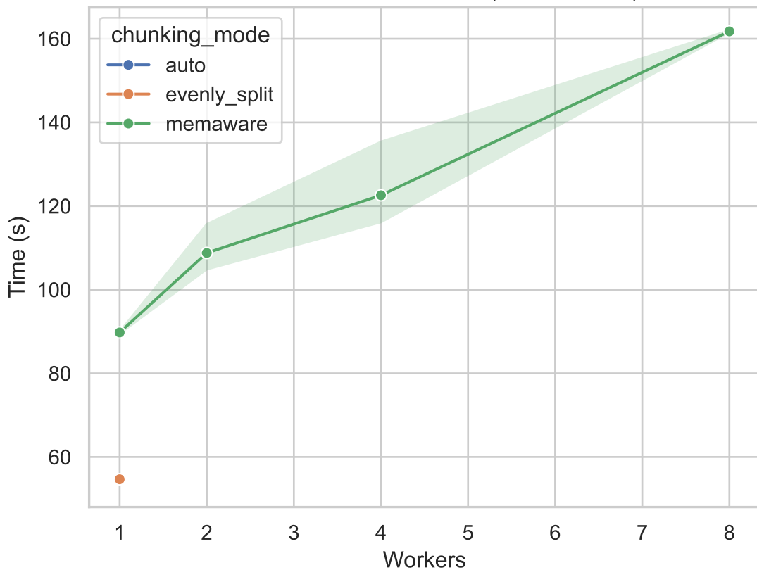
Execution Time vs Workers (400x300x300)
