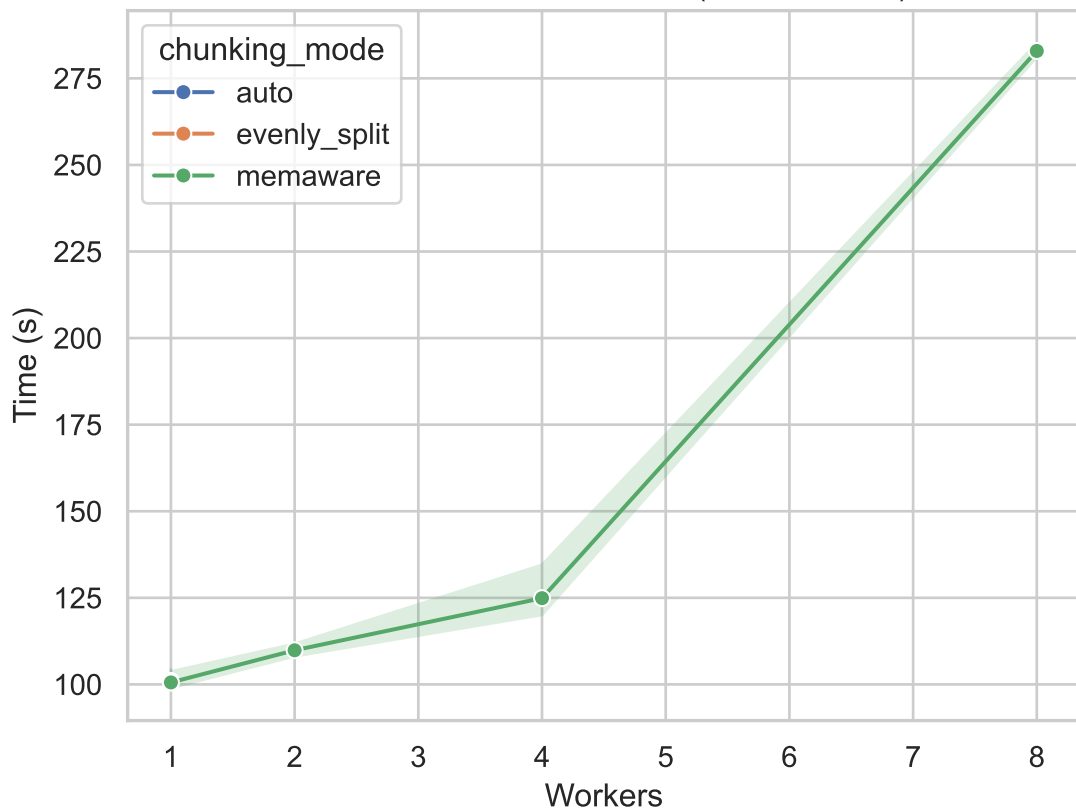
Execution Time vs Workers (400x400x400)
