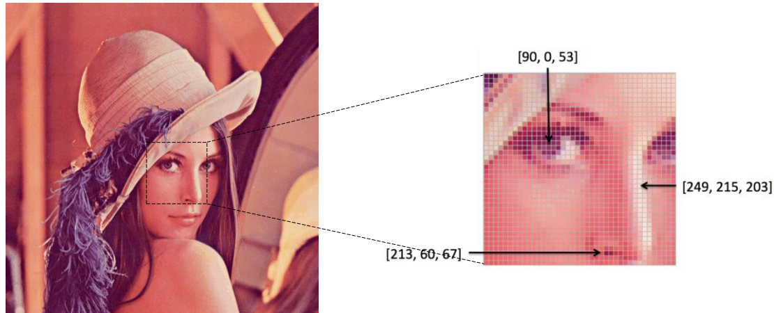
Lenna ( link )
