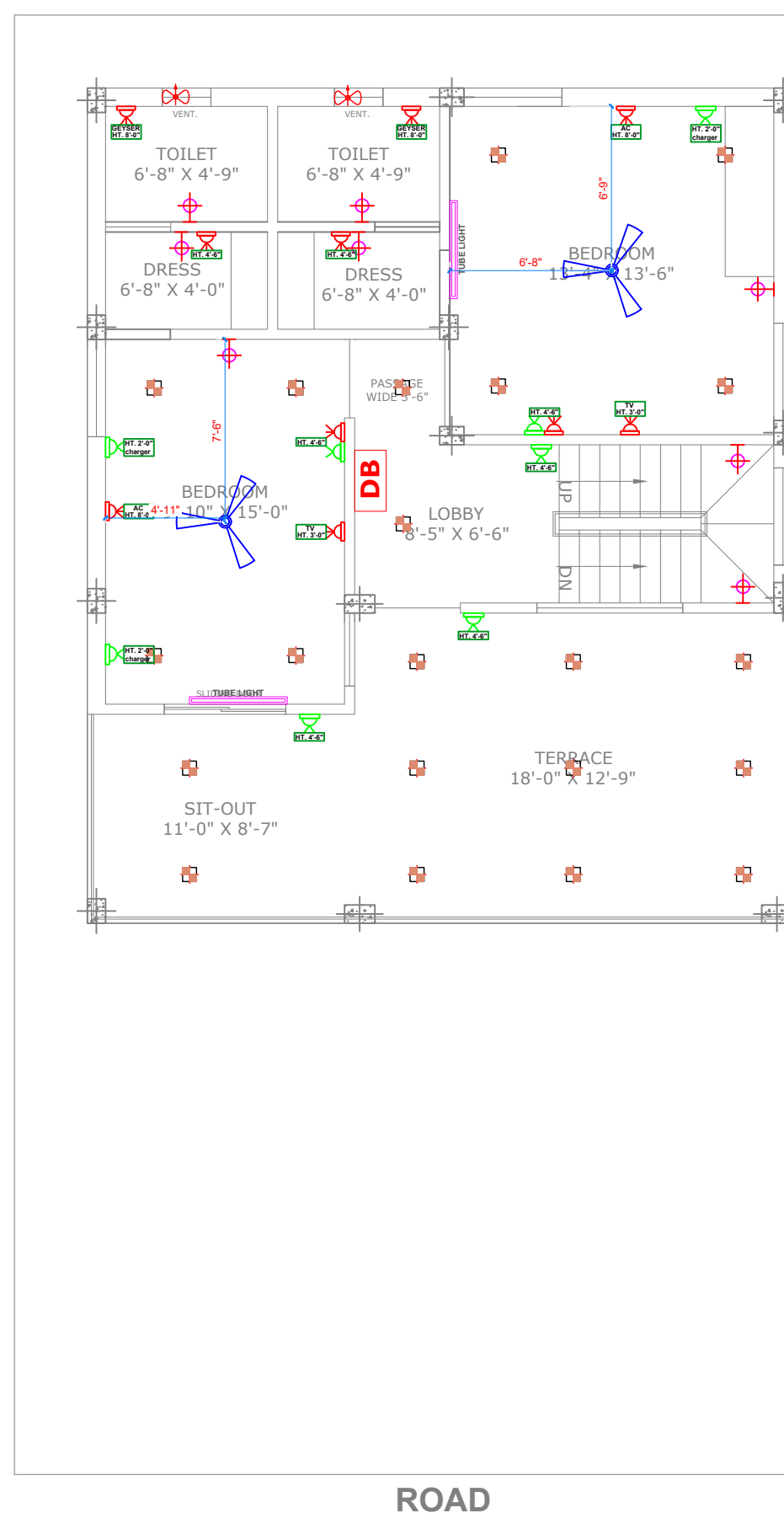
F.F.ELECTRICAL LAYOUT
