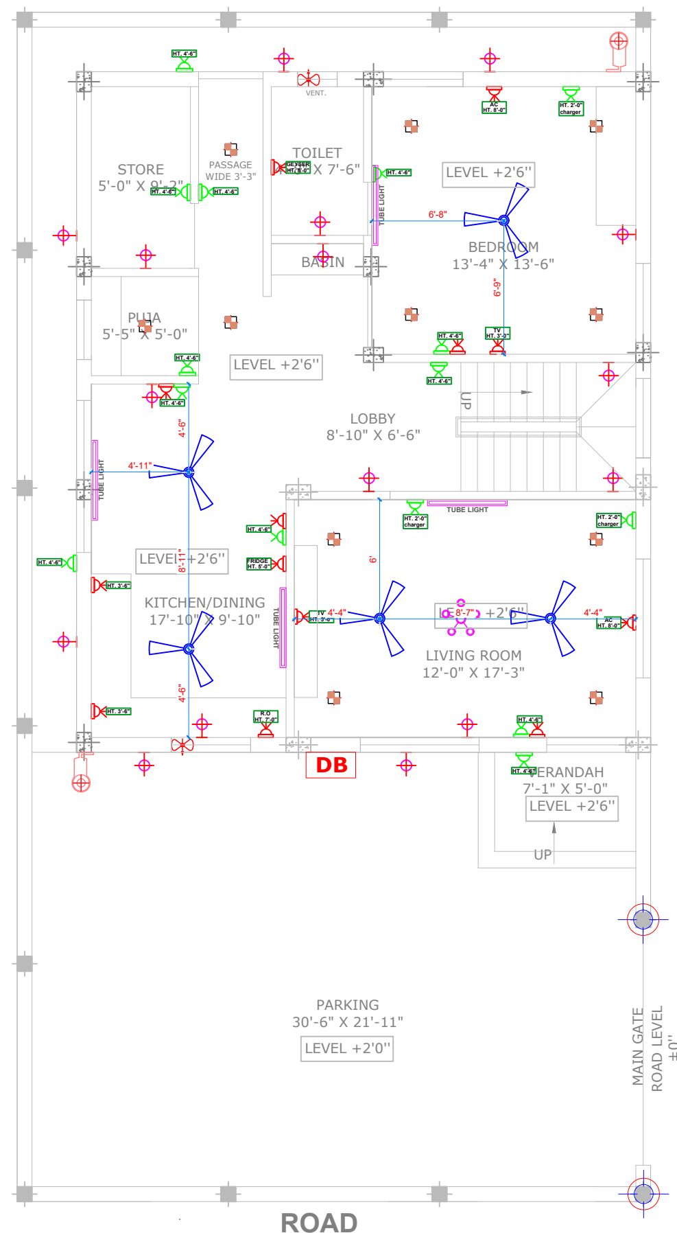
G.F.ELECTRICAL LAYOUT
