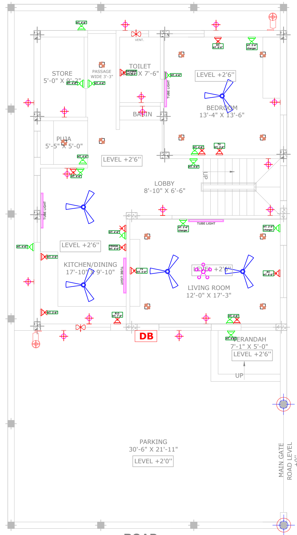
G.F.ELECTRICAL LAYOUT
