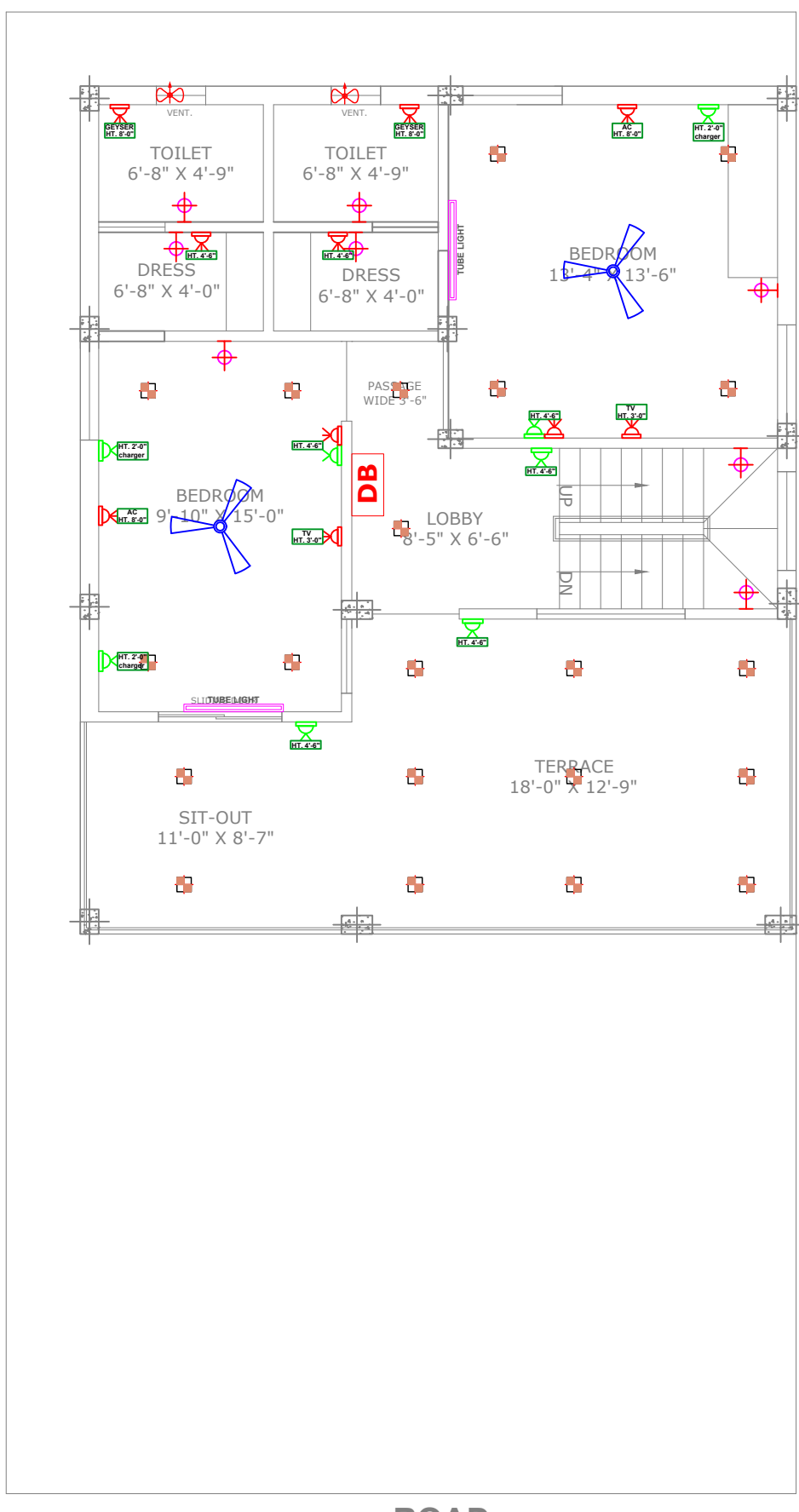
F.F.ELECTRICAL LAYOUT
