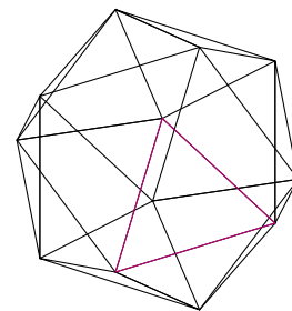
Figure 2: icosahedron
