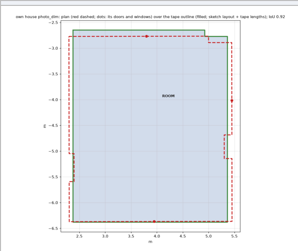
Figure 4. Own bedroom, 6 dim photos: 5/6 walls within 8%, footprint +0.6%
