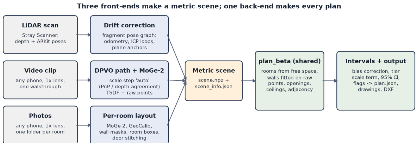
Figure 1. Architecture. Each tier only has to deliver a metric scene; the plan, the intervals and the drawings are shared.
