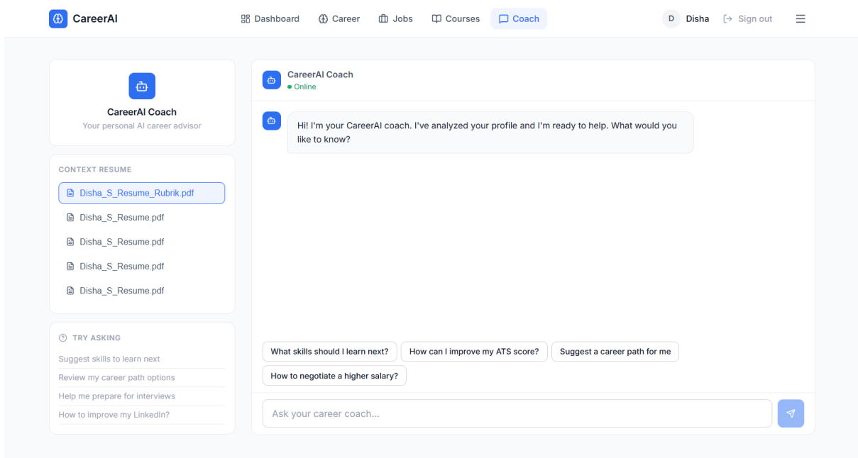
Fig 5: AI Career Coach — Conversational interface with resume context and quick prompts
