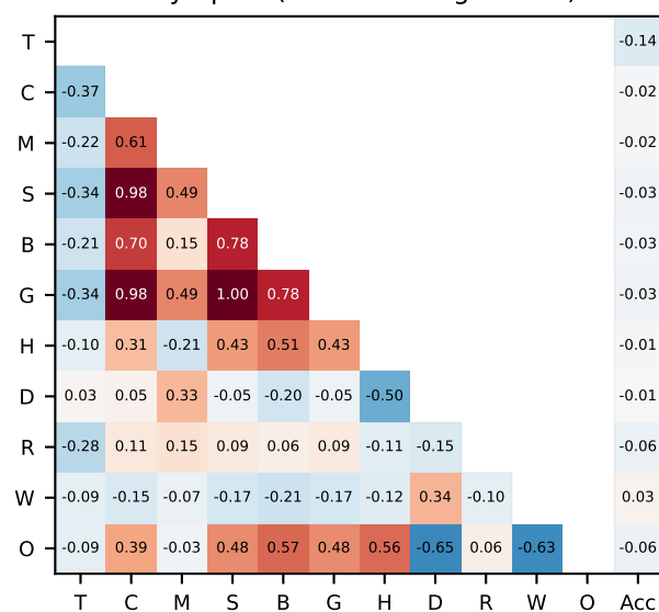
Olympiad (token-bearing n=615)
