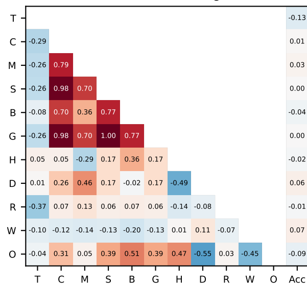
MATH-500 (token-bearing n=424)
