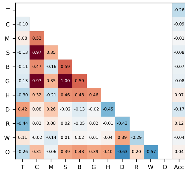
Olympiad (token-bearing n=387)
