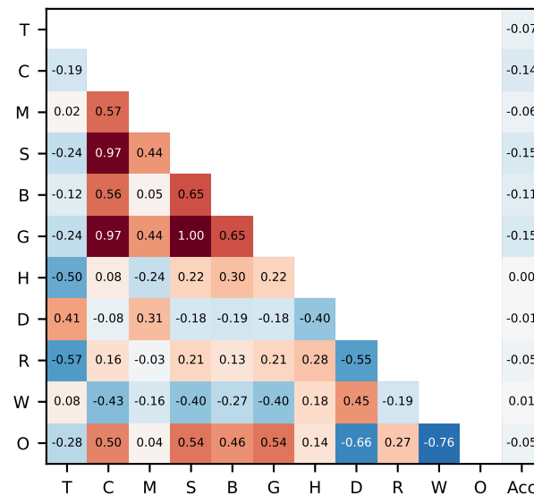
Minerva (token-bearing n=235)
