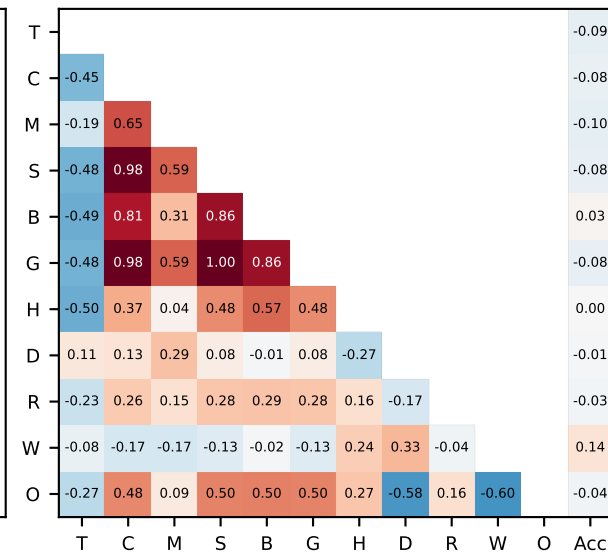
Minerva (token-bearing n=271)
