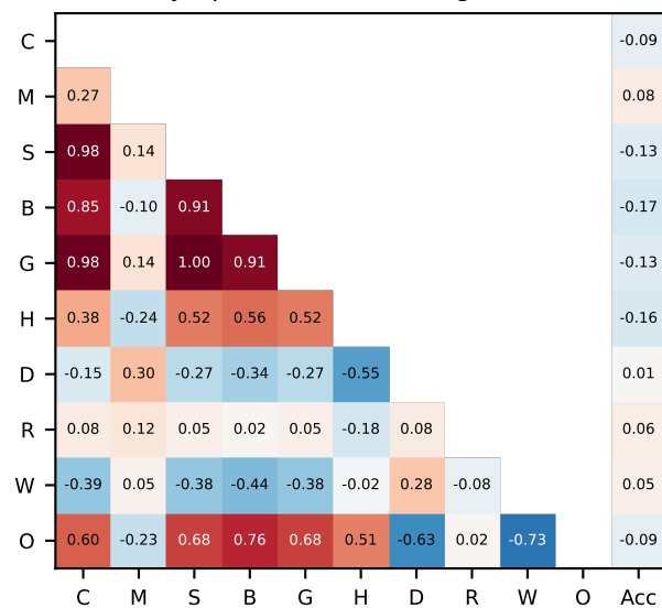
Olympiad (token-bearing n=407)
