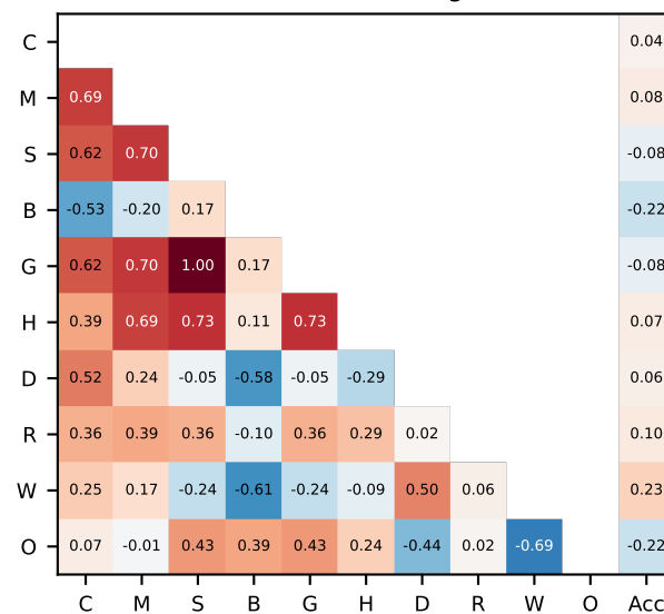
AIME25 (token-bearing n=942)
