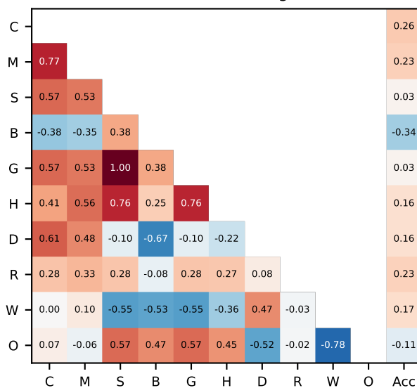
AIME24 (token-bearing n=948)
