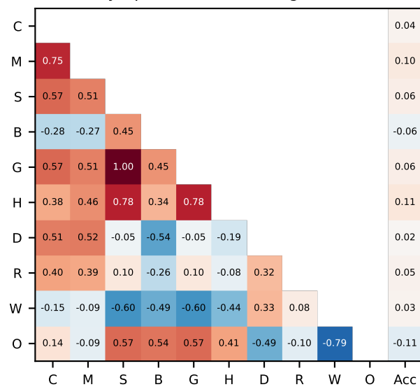
Olympiad (token-bearing n=209)
