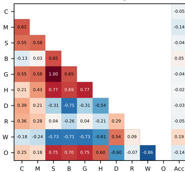
AMC23 (token-bearing n=176)
