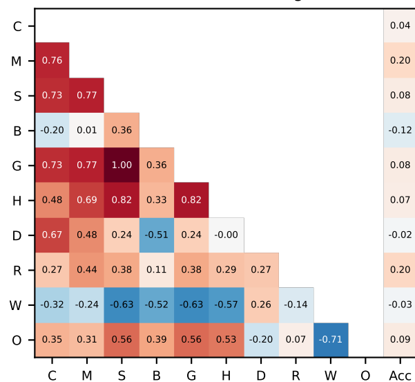
MATH-500 (token-bearing n=37)
