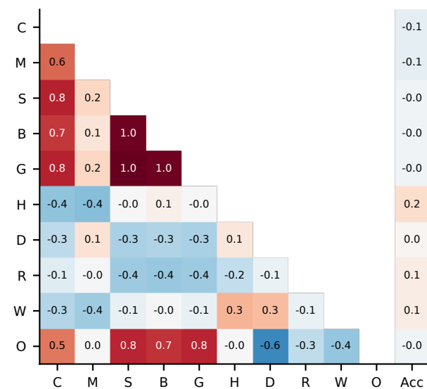
MATH-500
