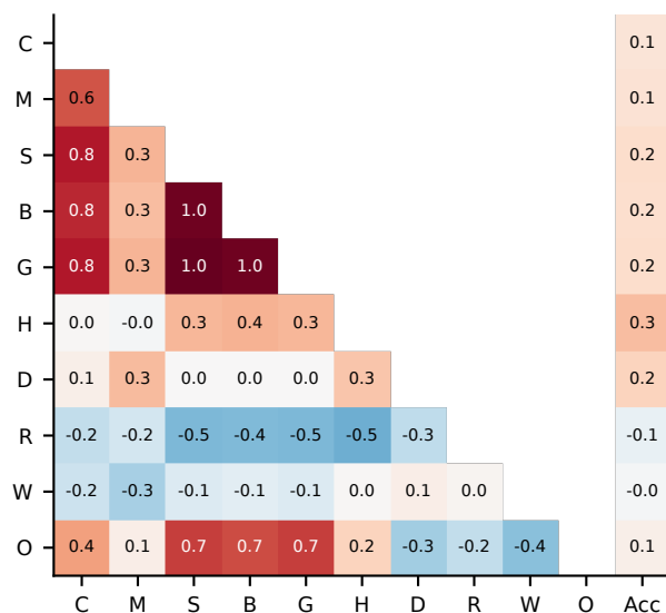
MATH-500
