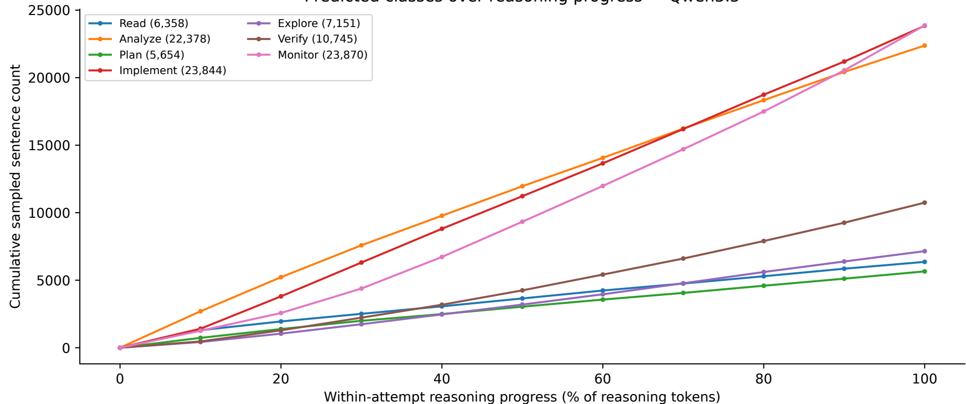
Predicted classes over reasoning progress — Qwen3.5
