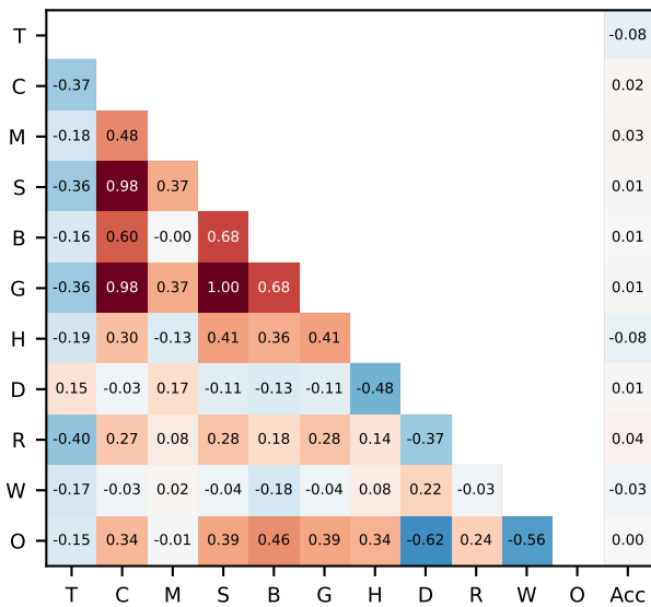
MATH-500 (token-bearing n=408)
