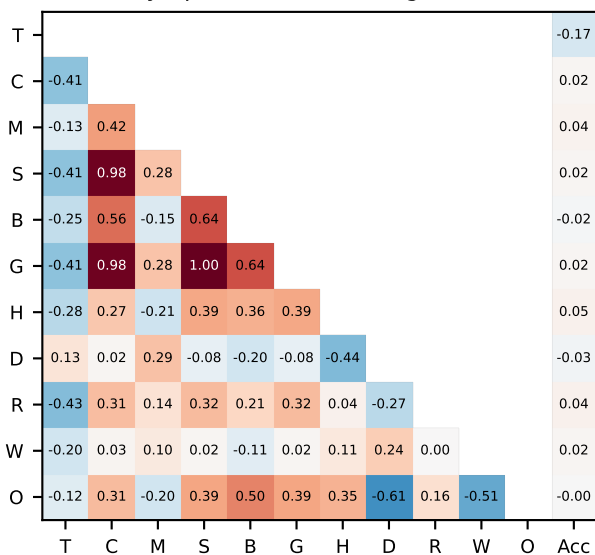
Olympiad (token-bearing n=597)
