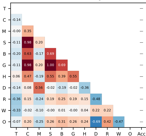
AMC23 (token-bearing n=37)
