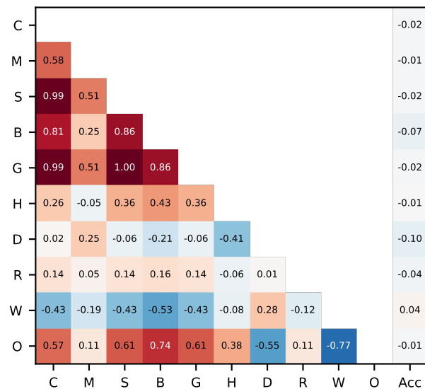
MATH-500 (token-bearing n=392)
