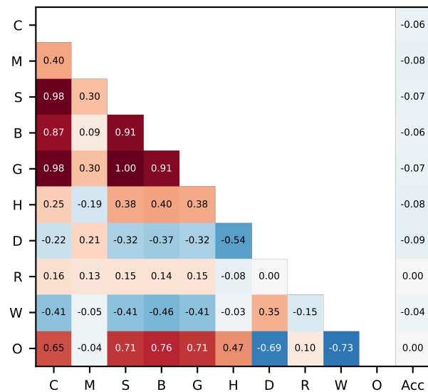
Olympiad (token-bearing n=655)
