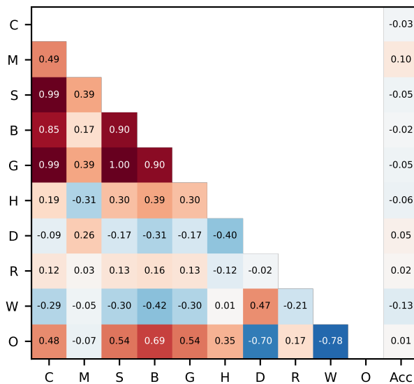
AMC23 (token-bearing n=1223)
