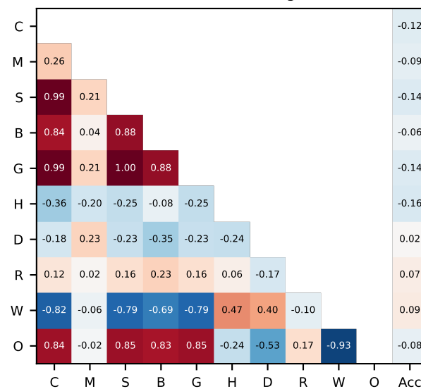
Minerva (token-bearing n=194)
