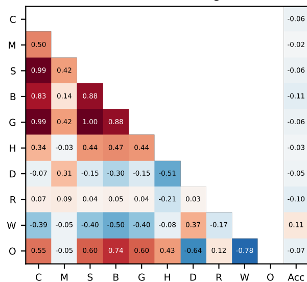
MATH-500 (token-bearing n=236)
