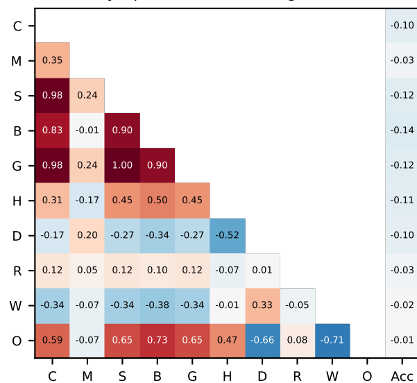
Olympiad (token-bearing n=526)
