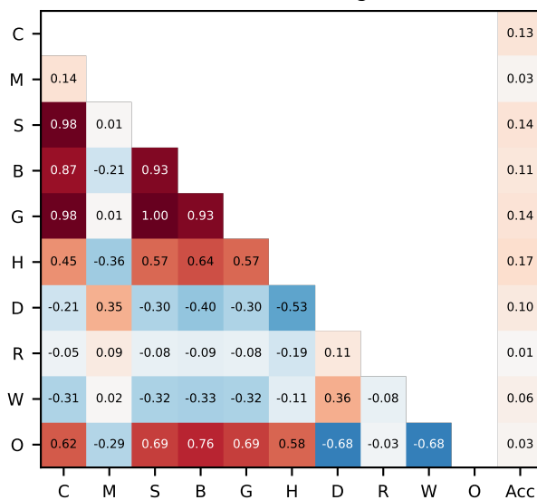
AMC23 (token-bearing n=787)
