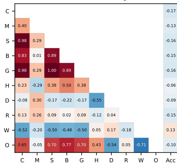
MATH-500 (token-bearing n=157)
