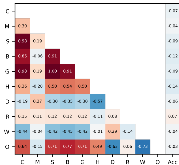
Olympiad (token-bearing n=438)
