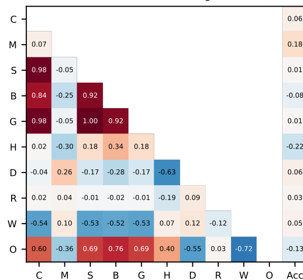
AIME25 (token-bearing n=834)
