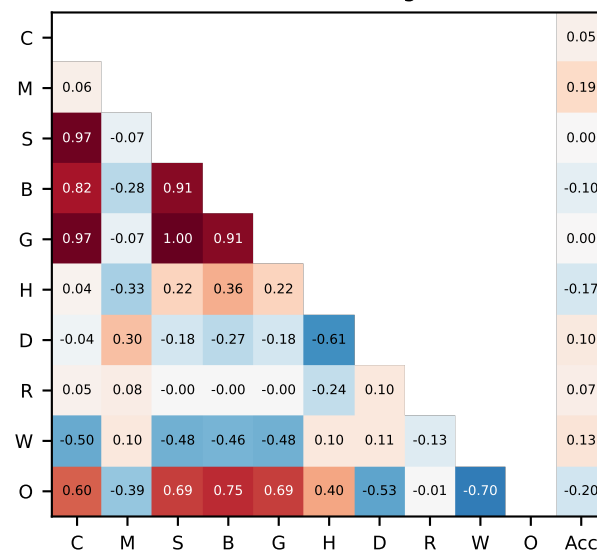
AIME25 (token-bearing n=770)
