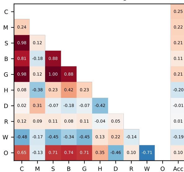
AIME24 (token-bearing n=719)
