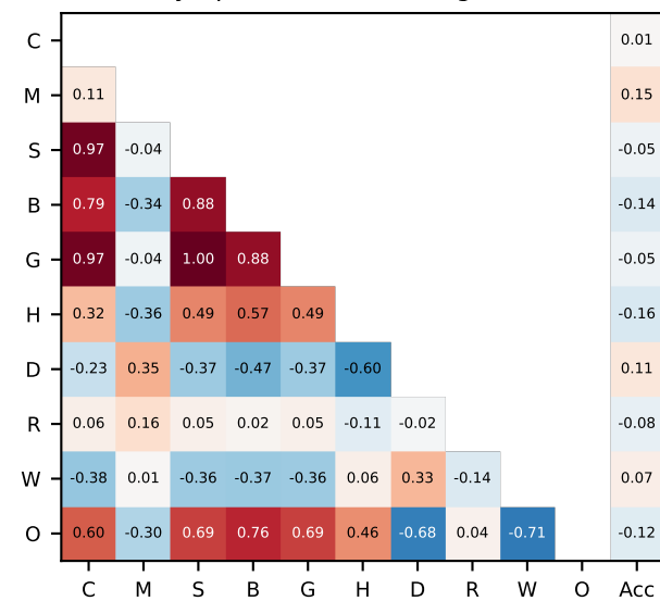
Olympiad (token-bearing n=316)
