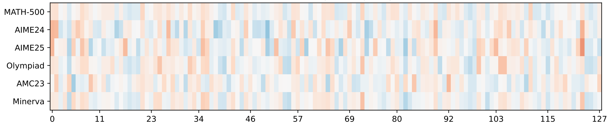
Gemma-4-26B-A4B: selected-expert frequency vs token count (rho)
