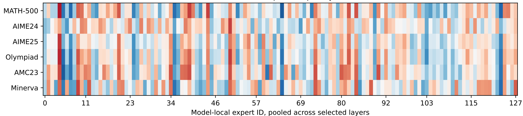
Gemma-4-26B-A4B: selected-expert frequency vs token count (rho)
