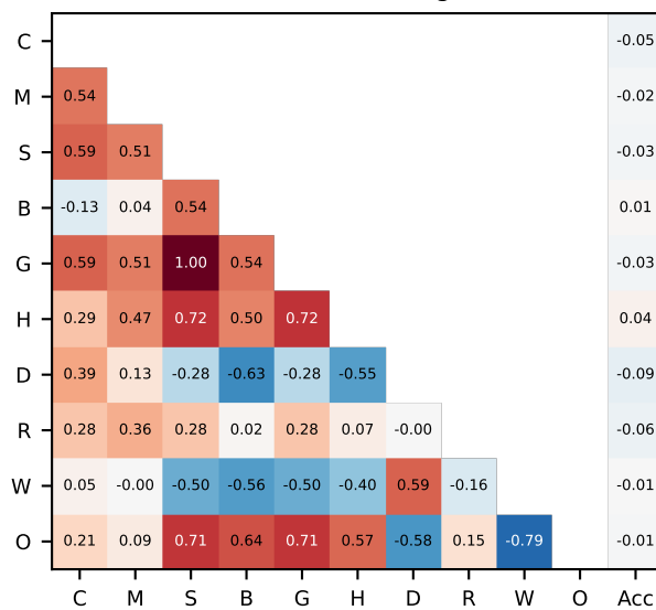
AMC23 (token-bearing n=666)
