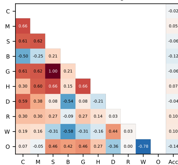
AIME25 (token-bearing n=864)
