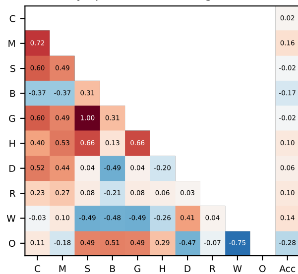
Olympiad (token-bearing n=398)
