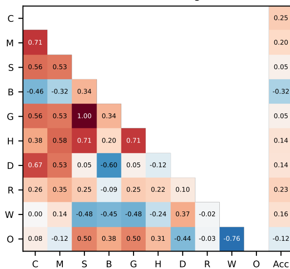
AIME24 (token-bearing n=853)
