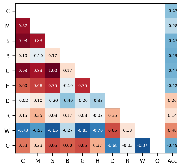
Minerva (token-bearing n=9)
