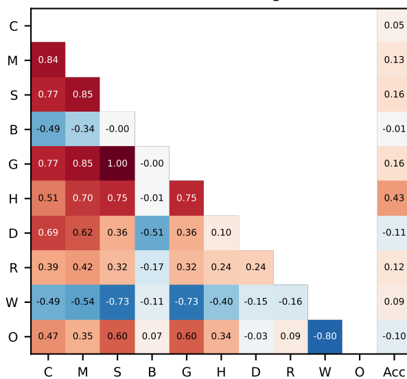
AIME24 (token-bearing n=383)
