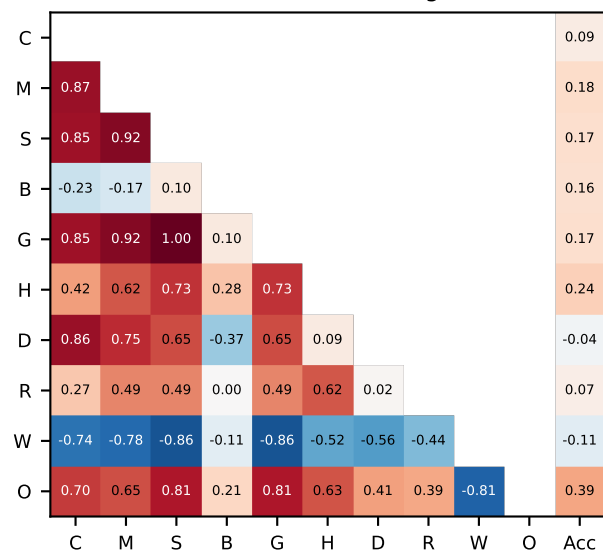
MATH-500 (token-bearing n=27)
