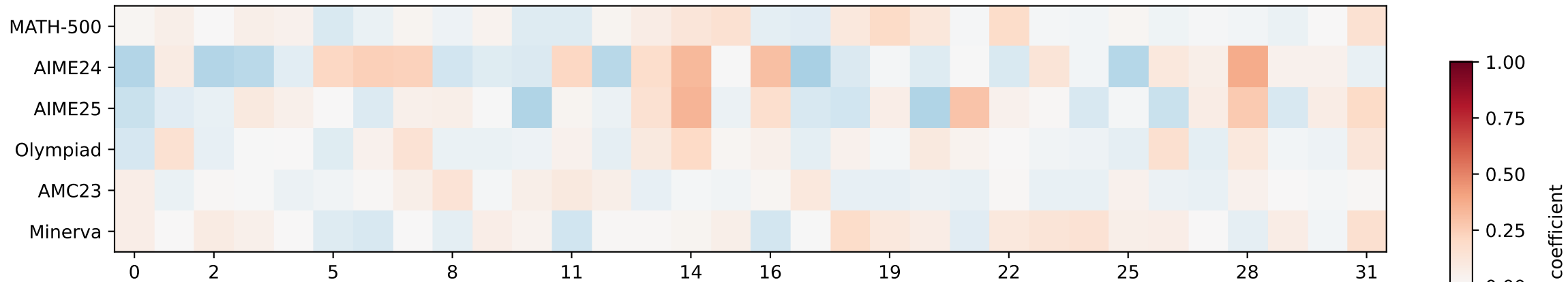
GPT-OSS-20B: selected-expert frequency vs token count (rho)
