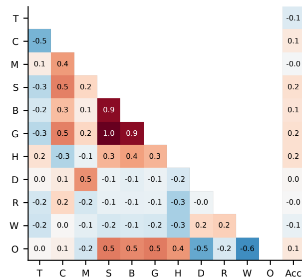
MATH-500
