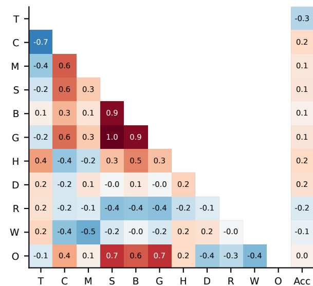
MATH-500
