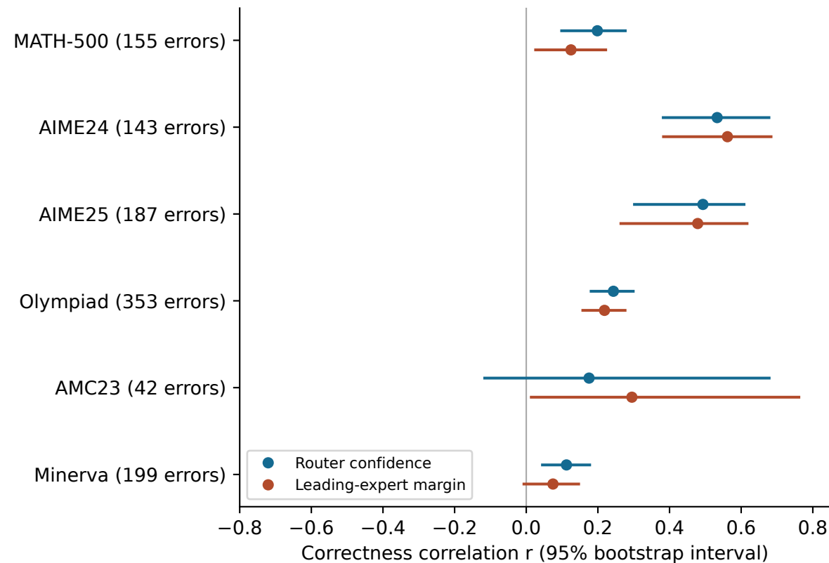
Whole continuation
