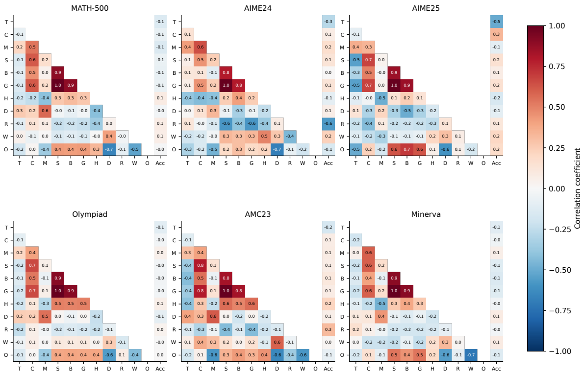
Fig. 27. Class: Read: metric relationships and correctness. Codes are defined in Table 47.
