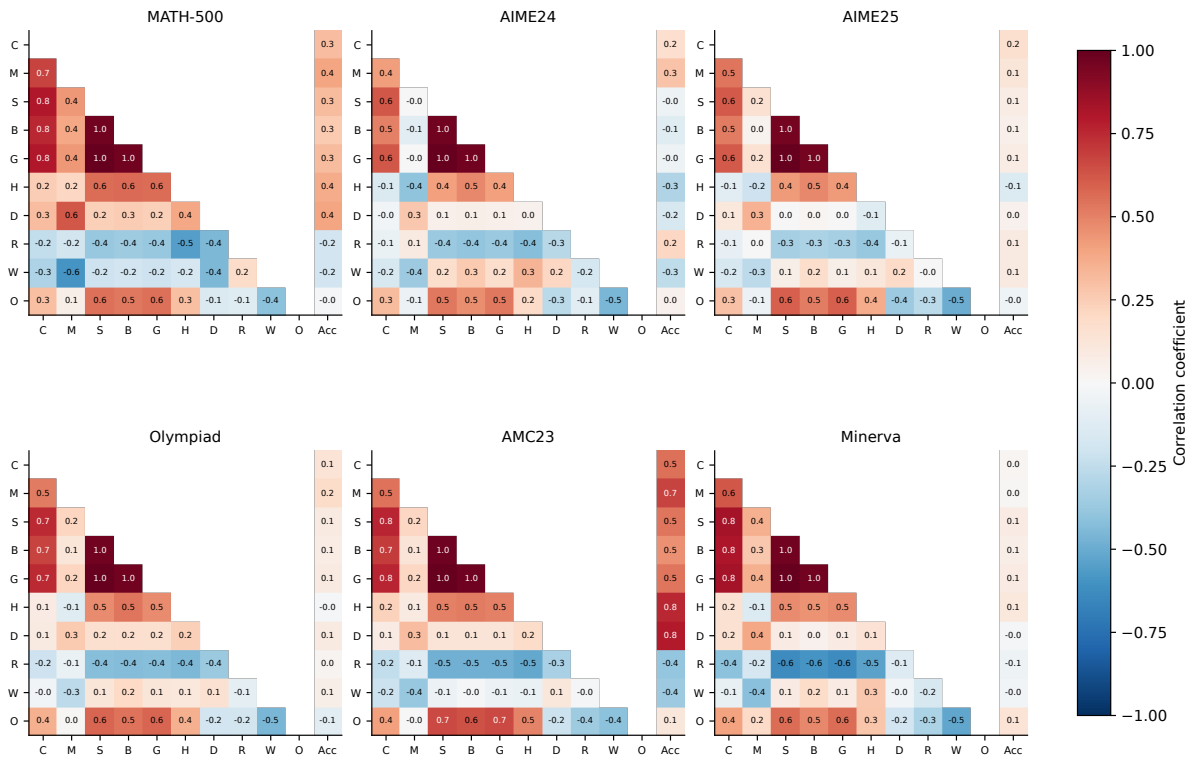
Fig. 41. Position: Bin 7: metric relationships and correctness. Codes are defined in Table 47.
