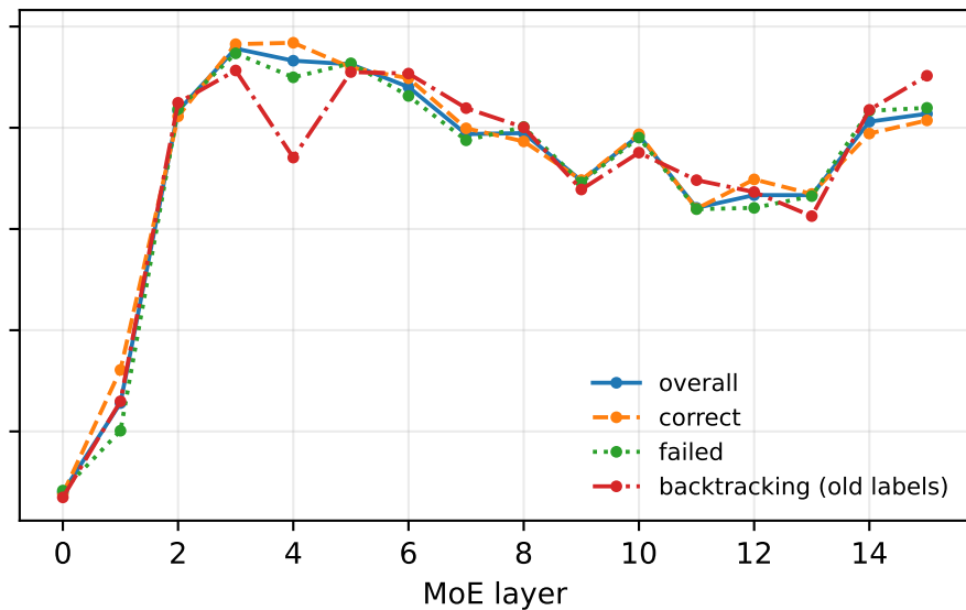
ProcessBench
