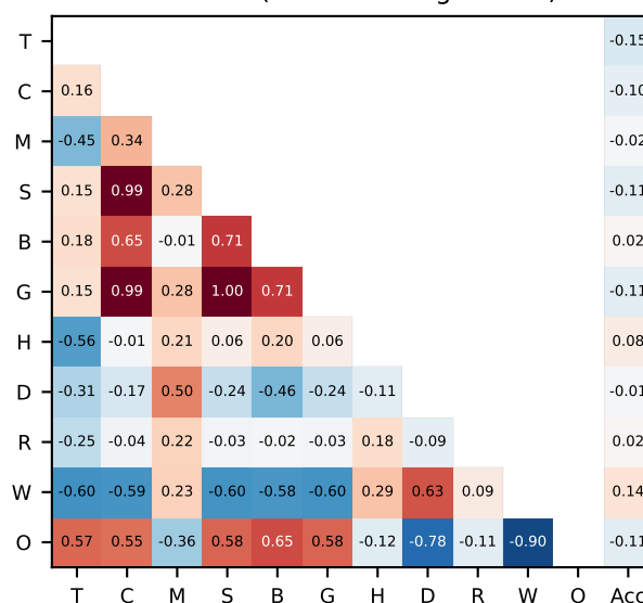
Minerva (token-bearing n=266)
