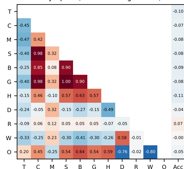
Olympiad (token-bearing n=639)
