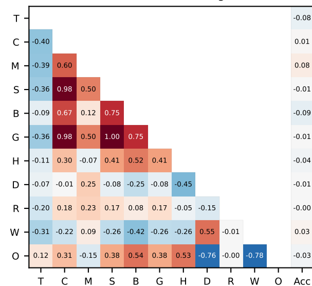
MATH-500 (token-bearing n=490)
