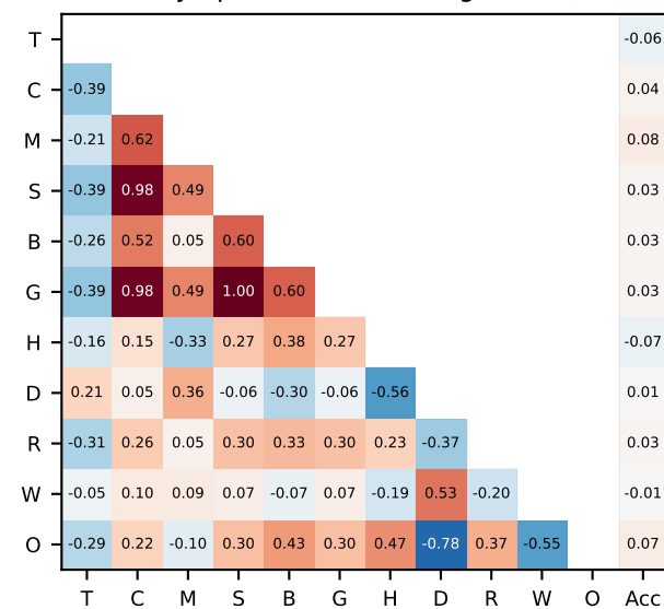
Olympiad (token-bearing n=542)
