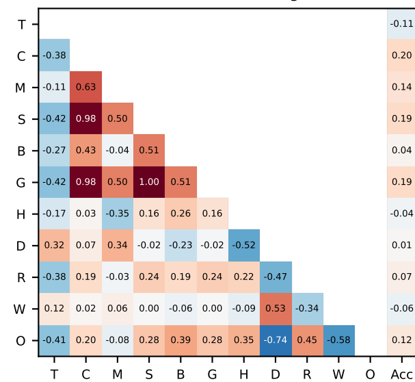
MATH-500 (token-bearing n=329)
