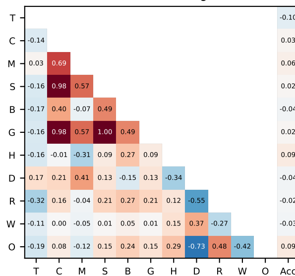
Minerva (token-bearing n=217)
