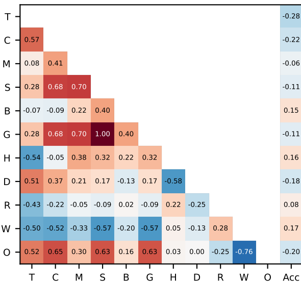
MATH-500 (token-bearing n=470)
