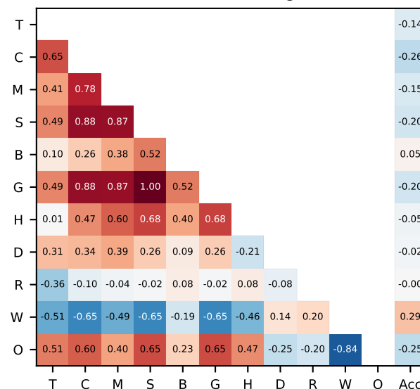
Minerva (token-bearing n=248)
