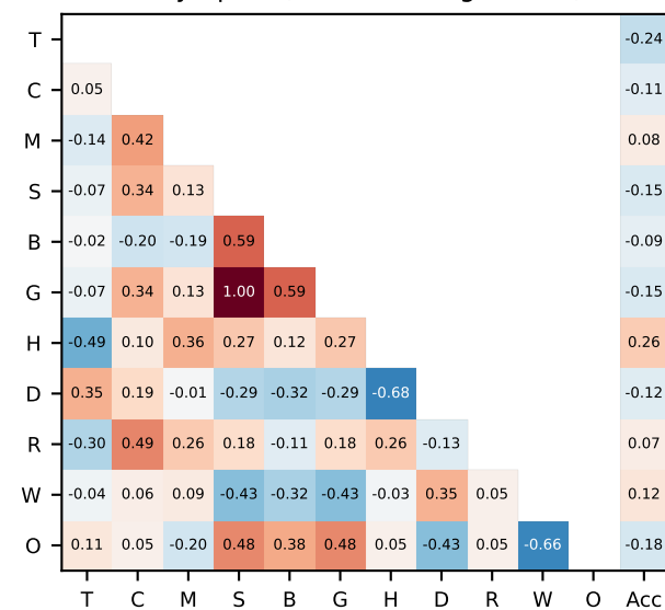
Olympiad (token-bearing n=517)
