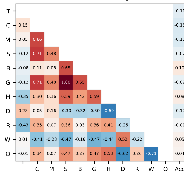
Minerva (token-bearing n=177)
