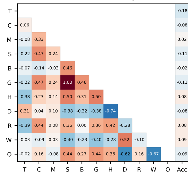
MATH-500 (token-bearing n=314)
