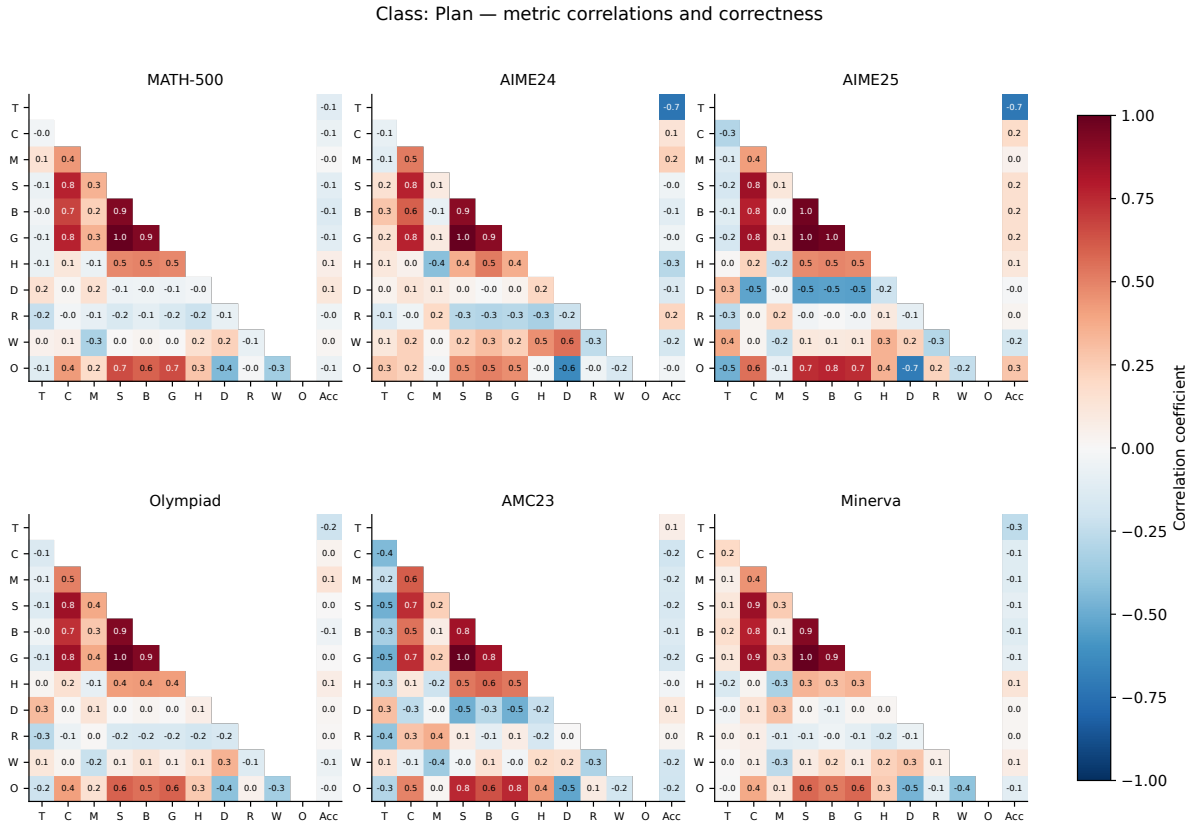
Fig. 29. Class: Plan: metric relationships and correctness. Codes are defined in Table 47.
