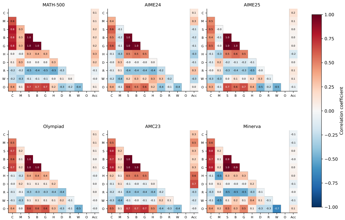
Fig. 39. Position: Bin 5: metric relationships and correctness. Codes are defined in Table 47.
