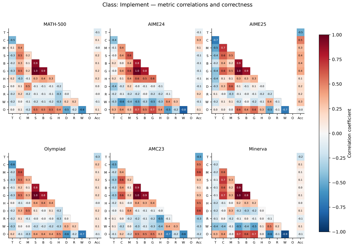
Fig. 30. Class: Implement: metric relationships and correctness. Codes are defined in Table 47.
