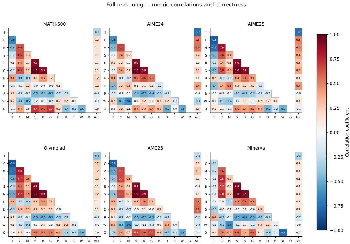
Fig. 26. Full reasoning: metric relationships and correctness. Codes are defined in Table 47.
