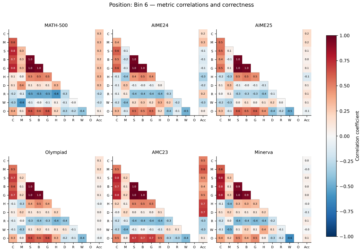
Fig. 40. Position: Bin 6: metric relationships and correctness. Codes are defined in Table 47.
