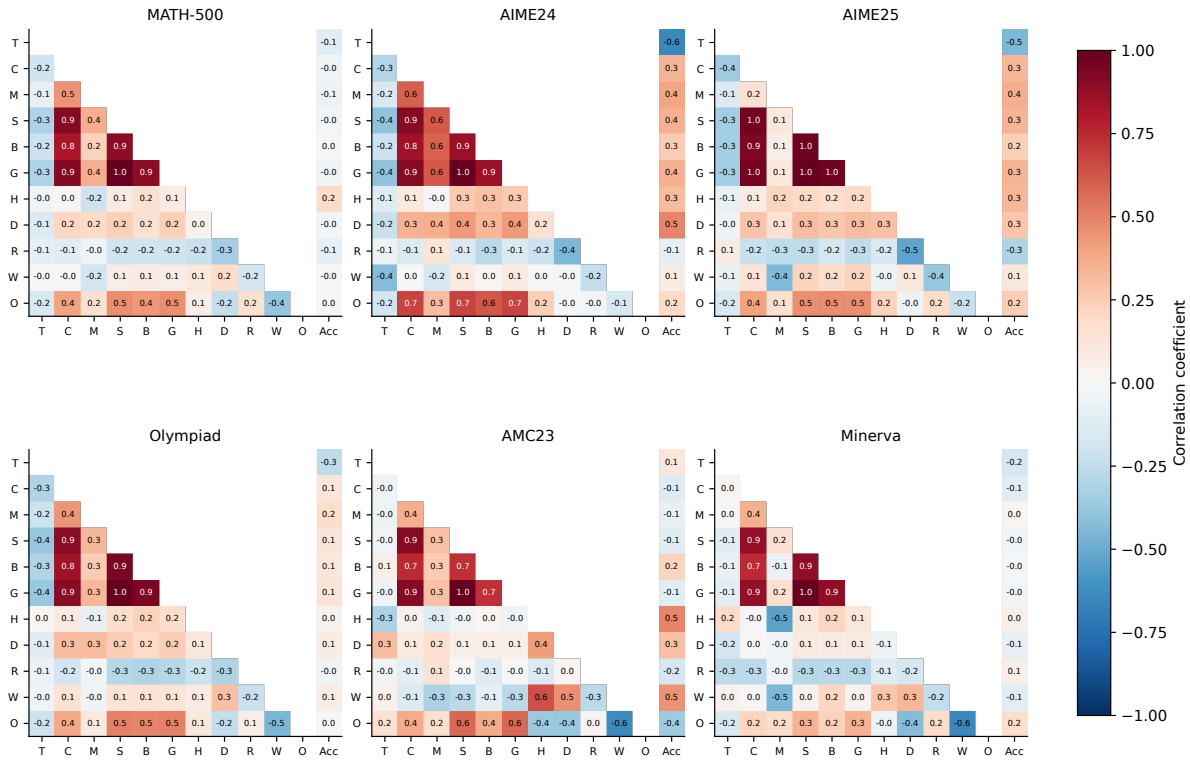
Fig. 31. Class: Explore: metric relationships and correctness. Codes are defined in Table 47.
