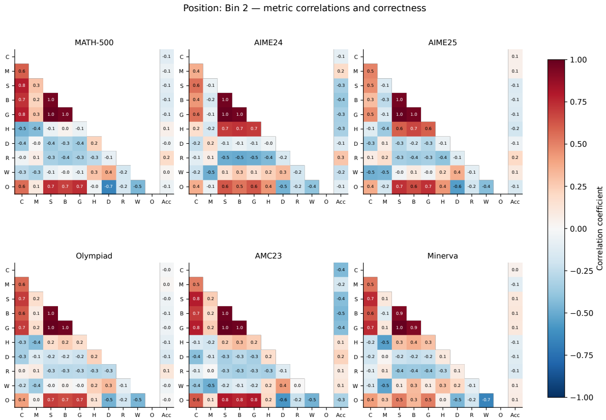
Fig. 36. Position: Bin 2: metric relationships and correctness. Codes are defined in Table 47.
