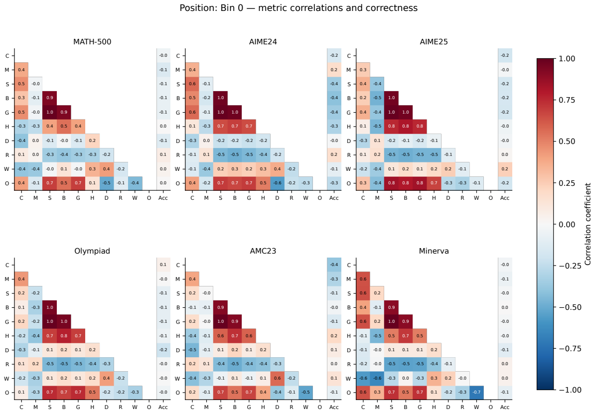
Fig. 34. Position: Bin 0: metric relationships and correctness. Codes are defined in Table 47.
