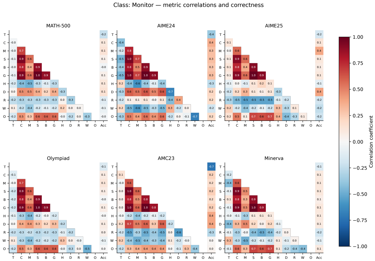
Fig. 33. Class: Monitor: metric relationships and correctness. Codes are defined in Table 47.
