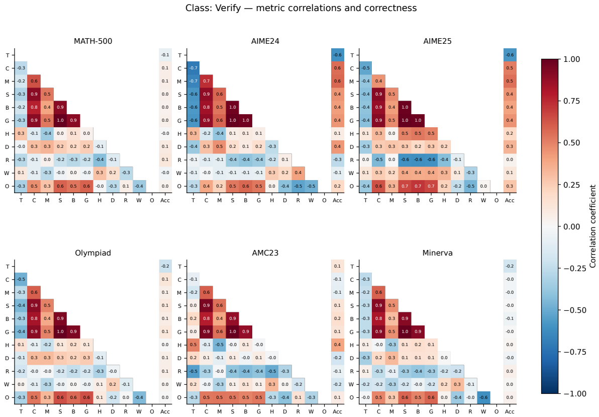
Fig. 32. Class: Verify: metric relationships and correctness. Codes are defined in Table 47.
