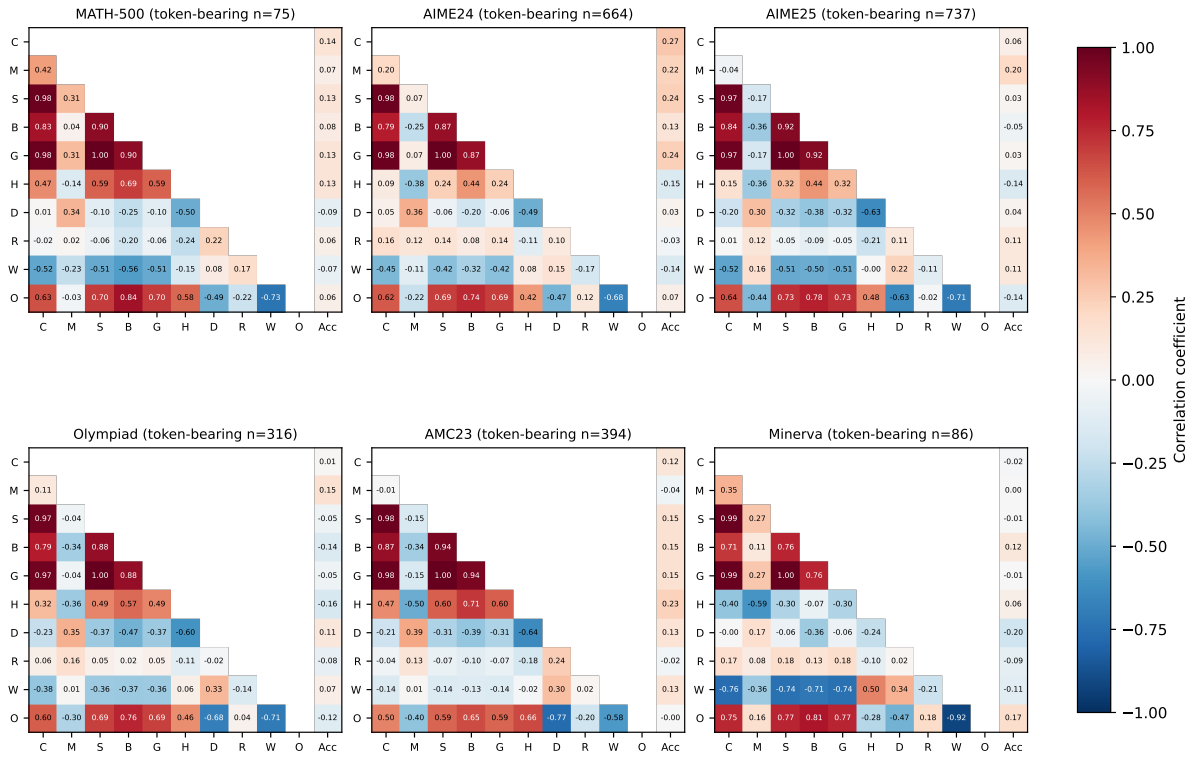
Fig. 63. Gemma-4-26B-A4B / Position: bin 09. Metric correlations and correctness; model-specific cohorts and tokenization.
