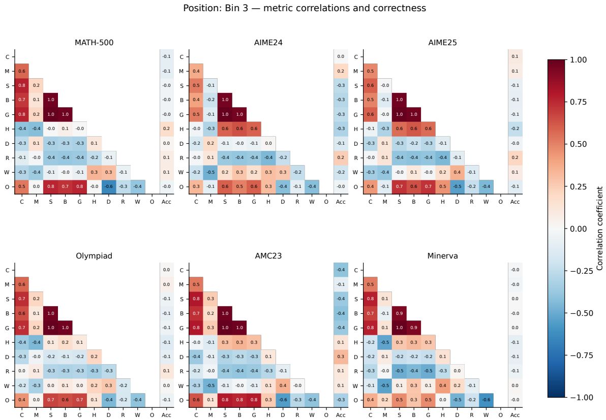
Fig. 37. Position: Bin 3: metric relationships and correctness. Codes are defined in Table 47.
