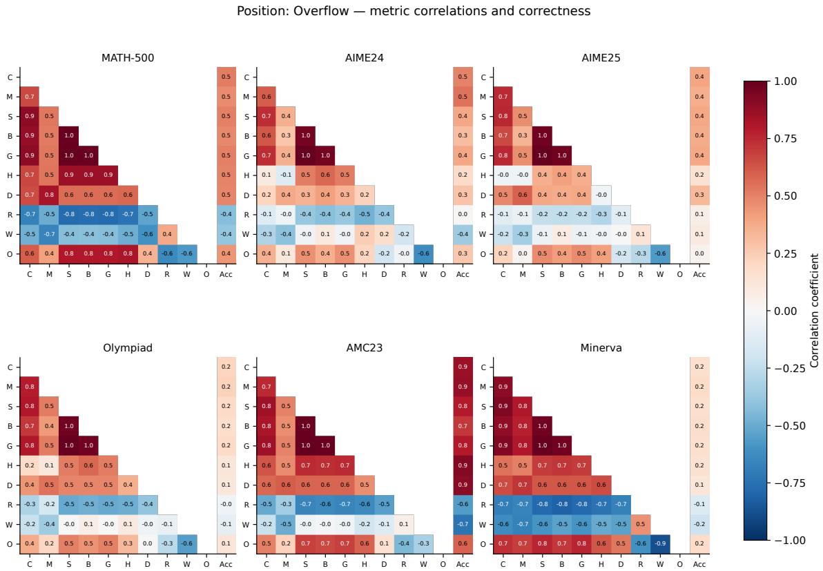
Fig. 44. Position: Overflow: metric relationships and correctness. Codes are defined in Table 47.
