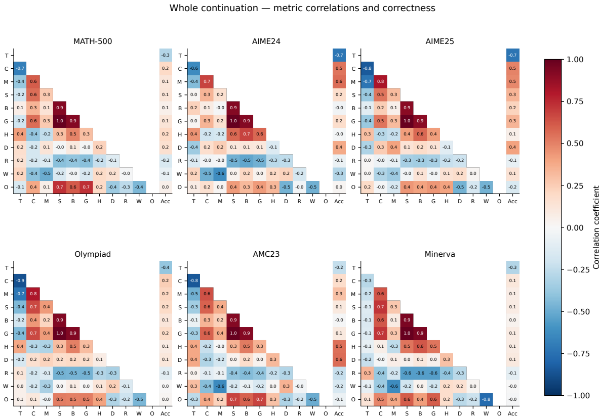
Fig. 25. Whole continuation: metric relationships and correctness. Codes are defined in Table 47.
