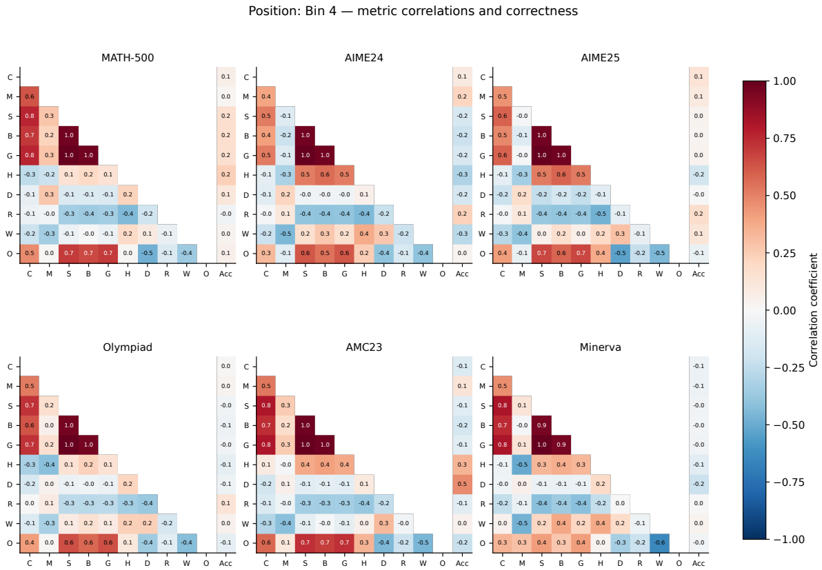
Fig. 38. Position: Bin 4: metric relationships and correctness. Codes are defined in Table 47.
