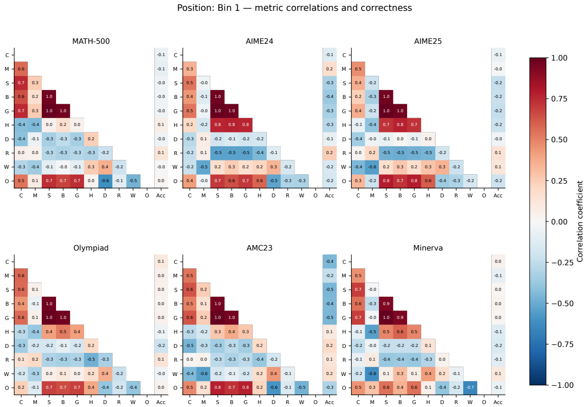
Fig. 35. Position: Bin 1: metric relationships and correctness. Codes are defined in Table 47.
