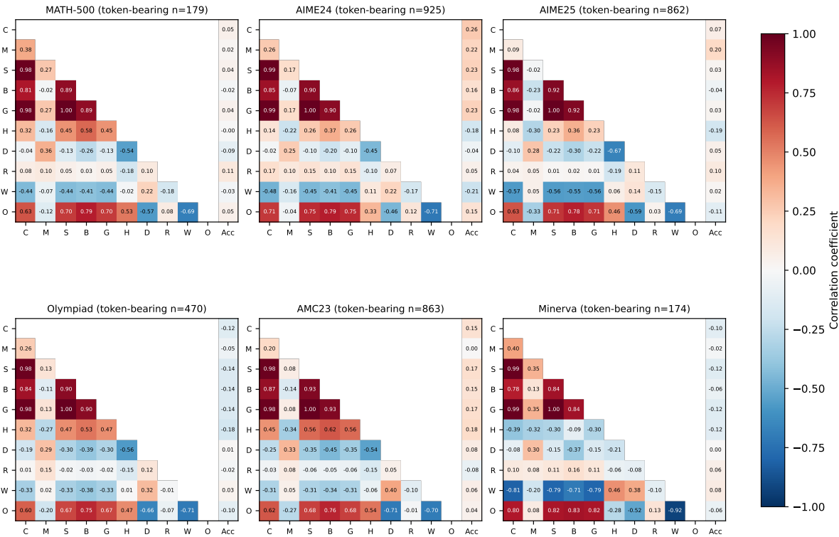
Fig. 58. Gemma-4-26B-A4B / Position: bin 04. Metric correlations and correctness; model-specific cohorts and tokenization.
