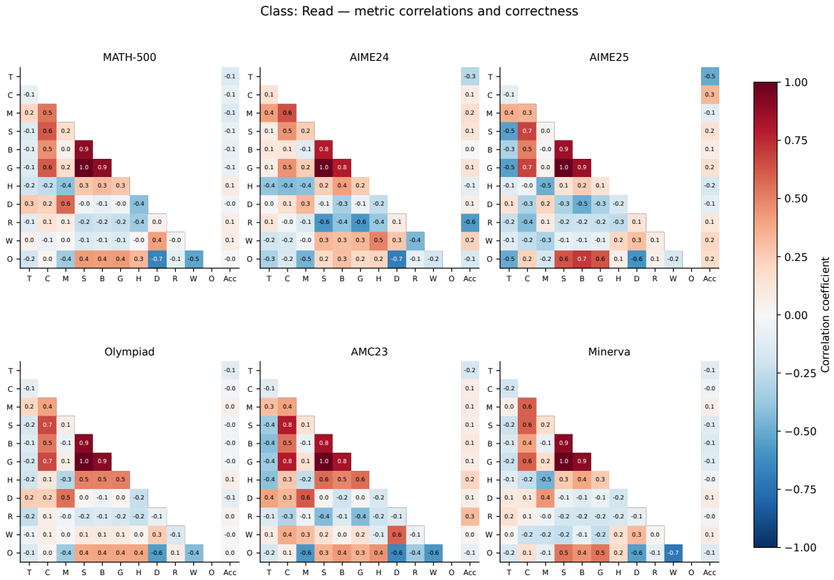
Fig. 27. Class: Read: metric relationships and correctness. Codes are defined in Table 47.
