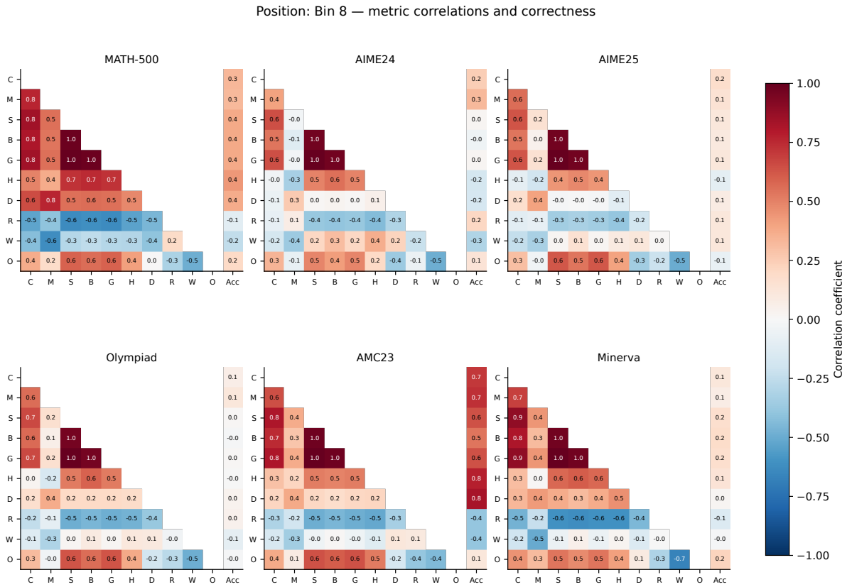
Fig. 42. Position: Bin 8: metric relationships and correctness. Codes are defined in Table 47.
