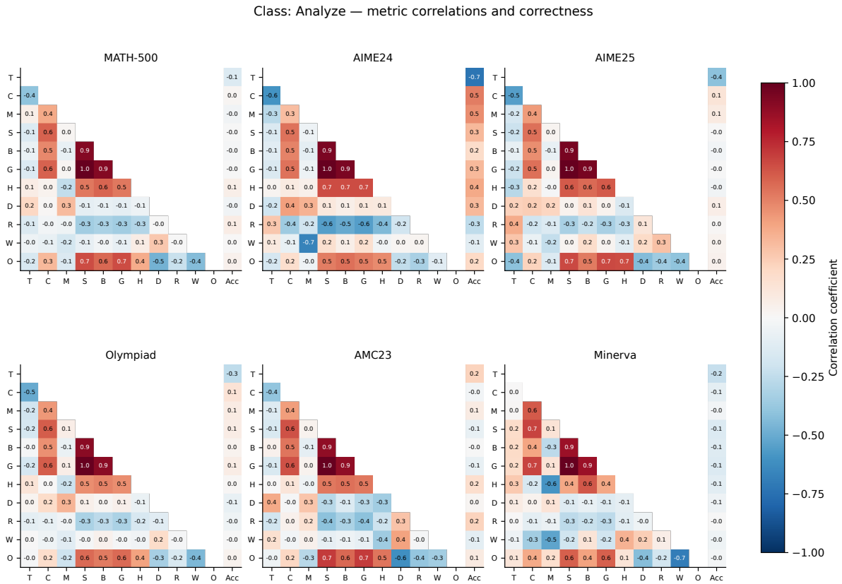
Fig. 28. Class: Analyze: metric relationships and correctness. Codes are defined in Table 47.
