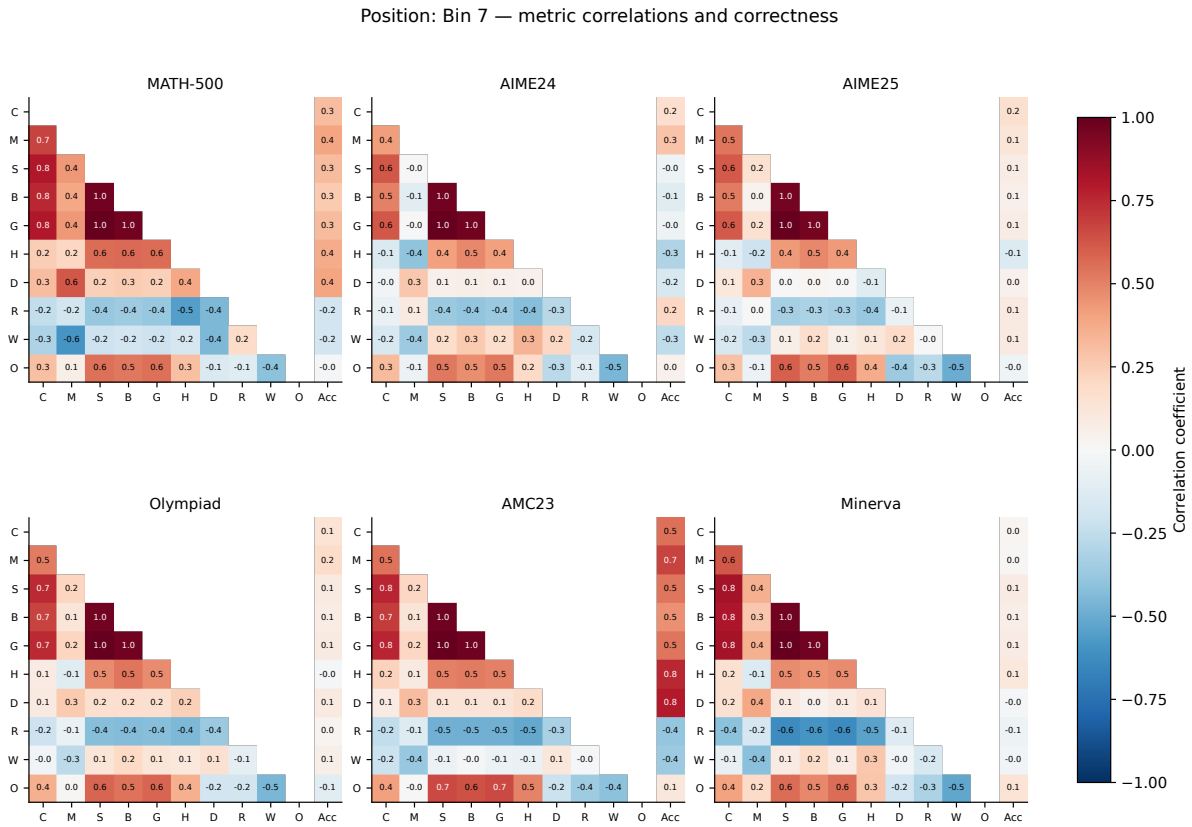
Fig. 41. Position: Bin 7: metric relationships and correctness. Codes are defined in Table 47.
