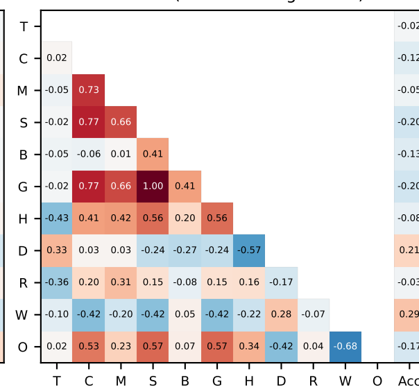
Minerva (token-bearing n=216)
