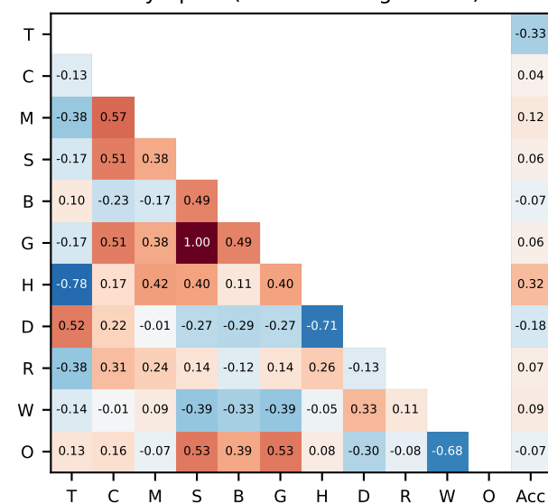
Olympiad (token-bearing n=587)
