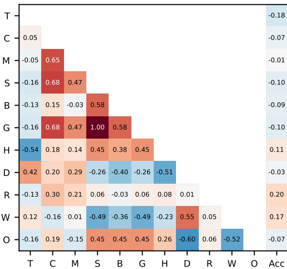
MATH-500 (token-bearing n=212)
