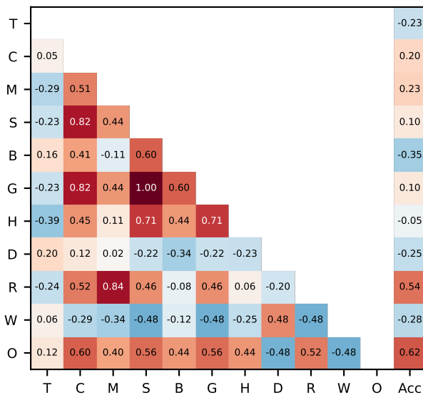
AMC23 (token-bearing n=19)
