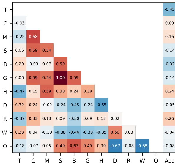
AIME24 (token-bearing n=27)
