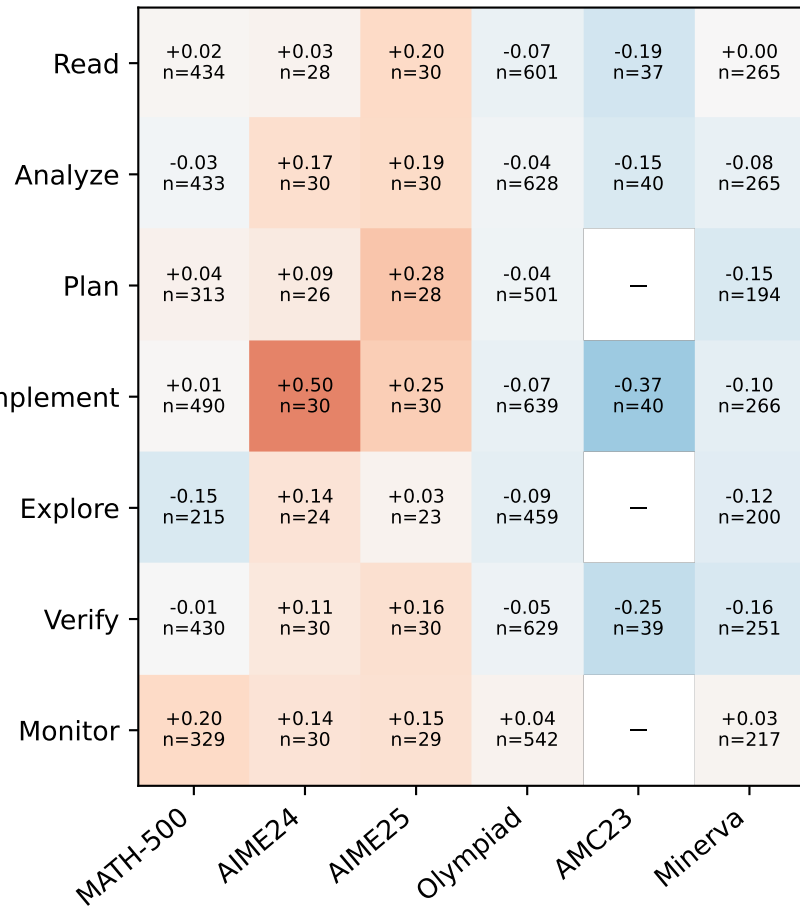
Gemma: class-conditioned confidence
