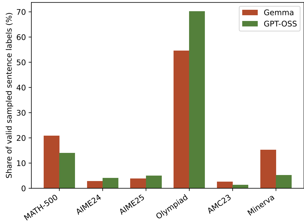
Benchmark composition
