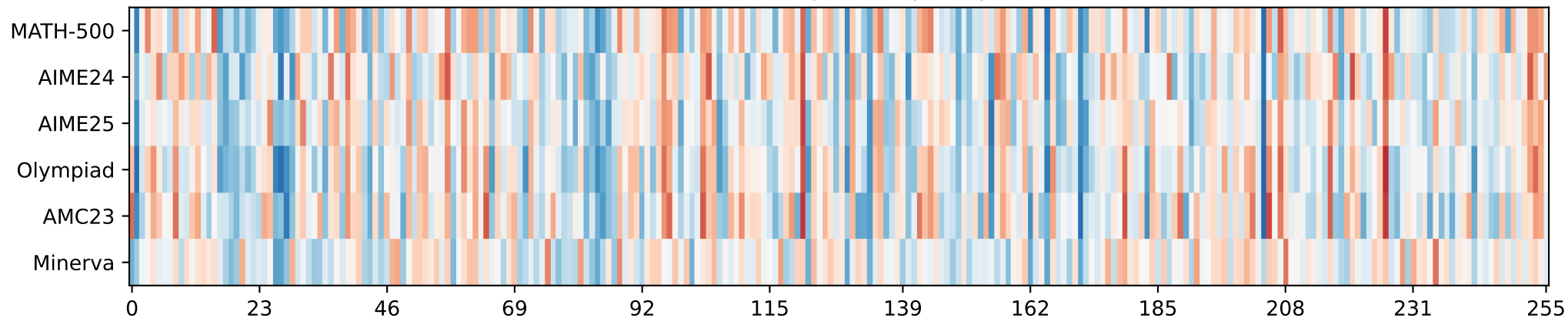
Qwen3.5-35B-A3B: selected-expert frequency vs token count (rho)
