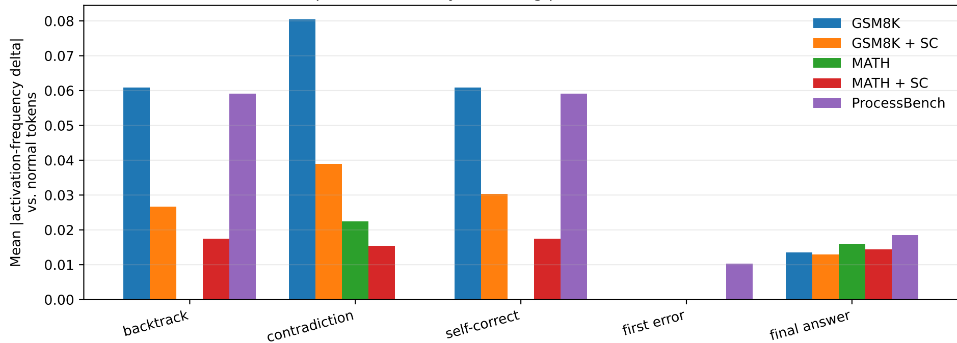
Expert-use shifts by reasoning phase (corrected labels)
