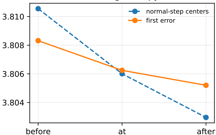
Routing entropy
