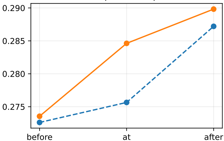
Top-k overlap
