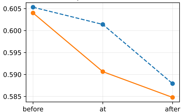
Expert-switch rate
