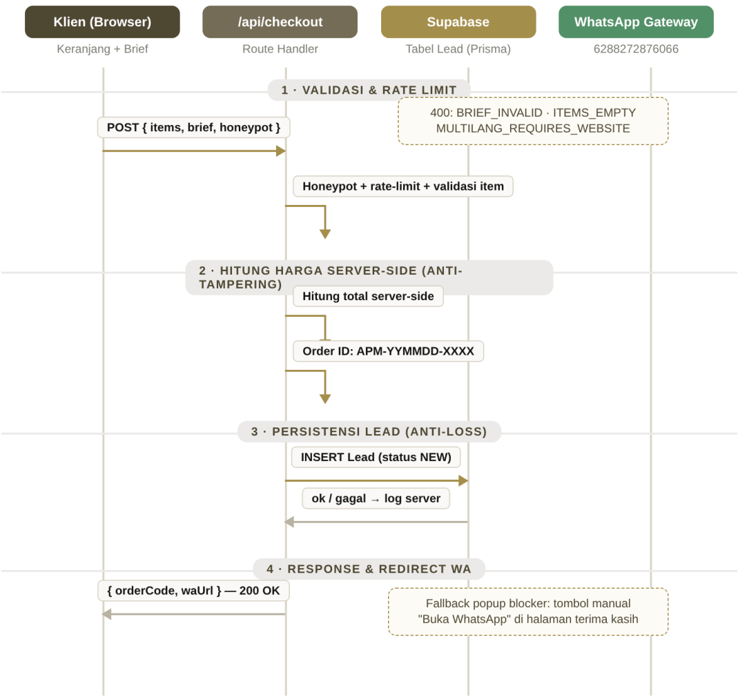
Gambar 5: Sequence diagram checkout — validasi, hitung harga server-side, persistensi Lead, redirect WhatsApp
