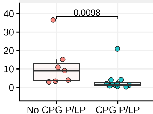
MB, SHH
