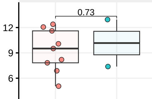
MB, WNT
