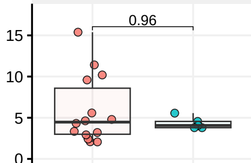
MB, Group3
