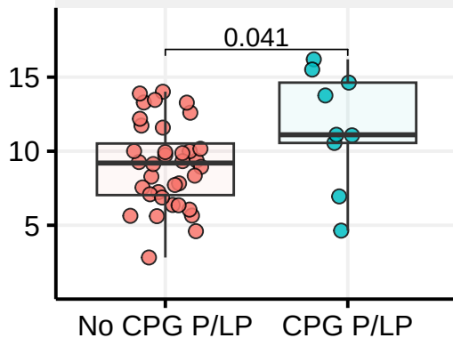
MB, Group4
