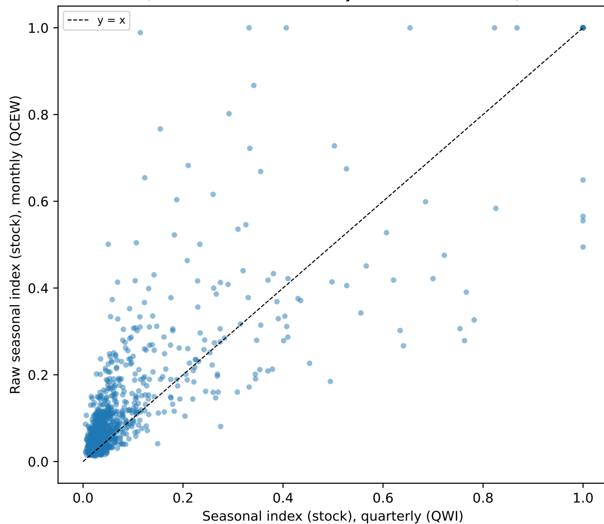
Raw comparison (conflates real seasonality with two confounds)
