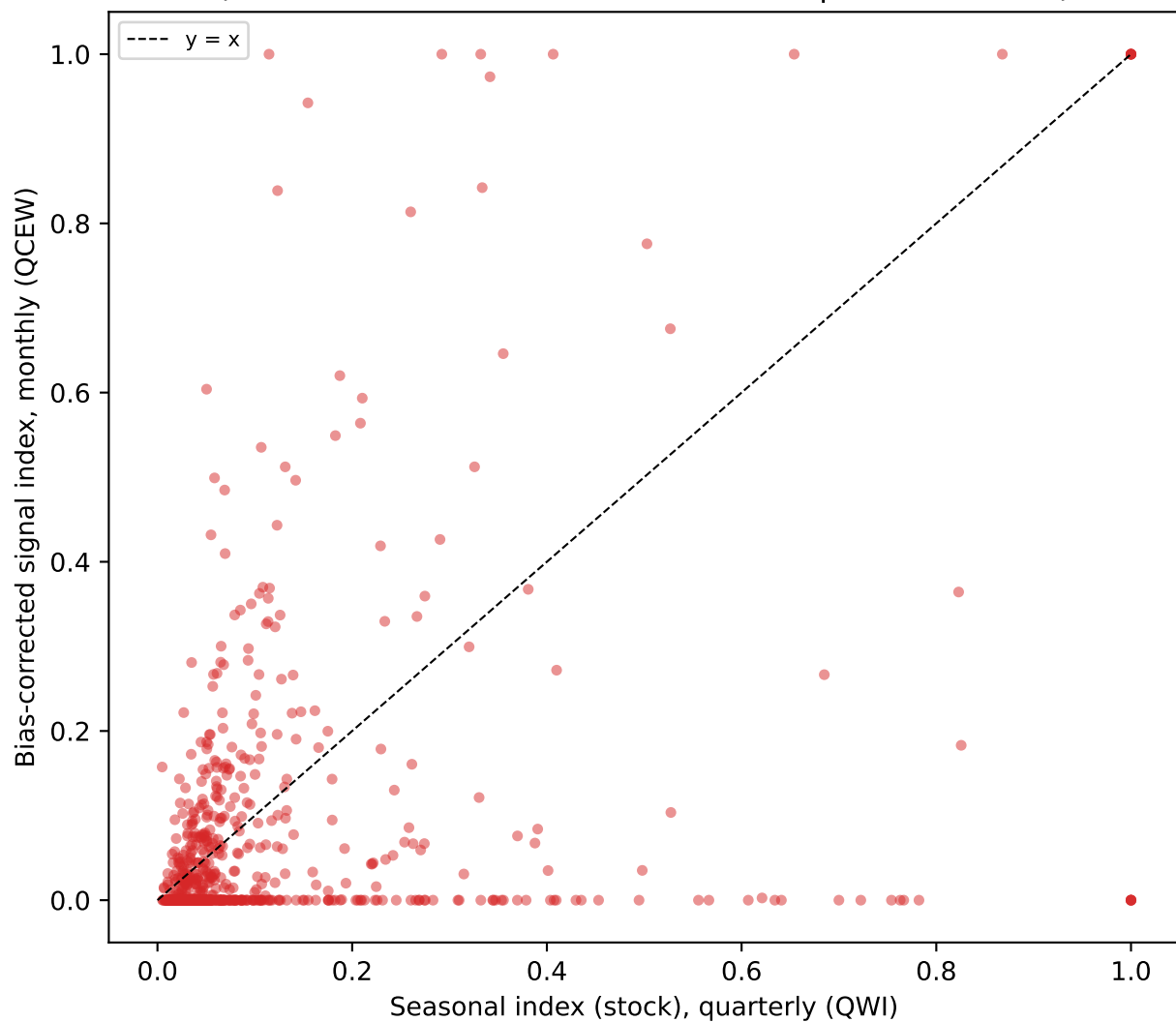
Bias-corrected comparison (net of common calendar effect + sample-size artifact)
