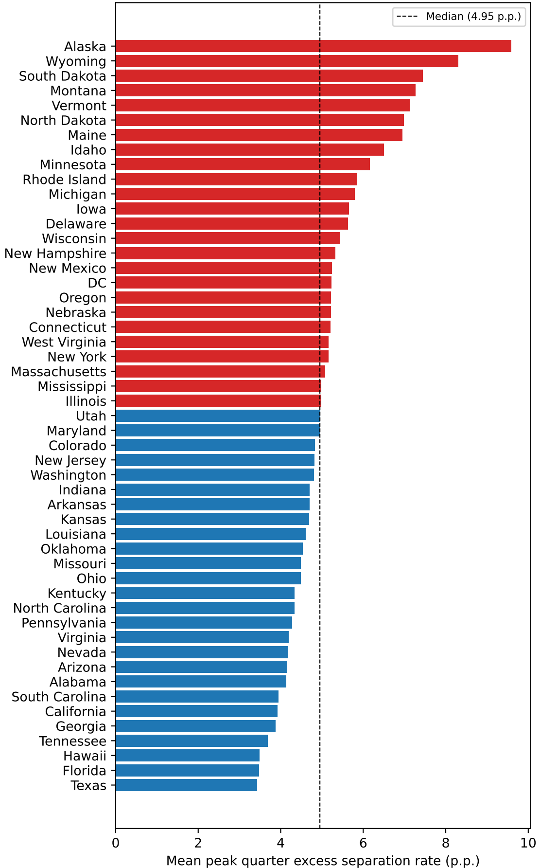
State-level seasonality (mean peak excess across 6-digit NAICS industries)
